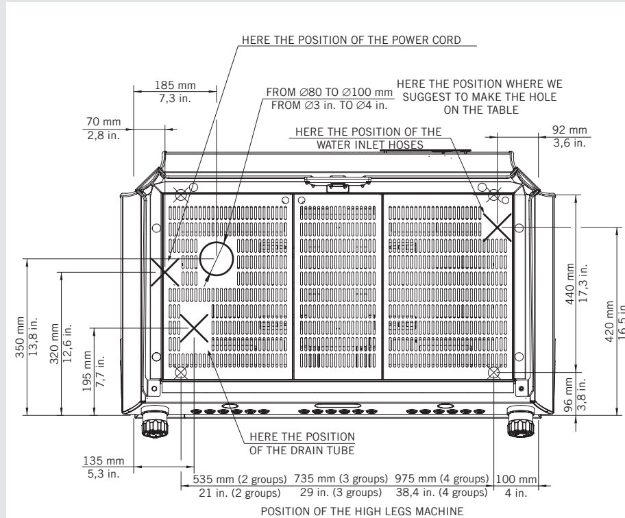
Fig. 2 - Installation guide
